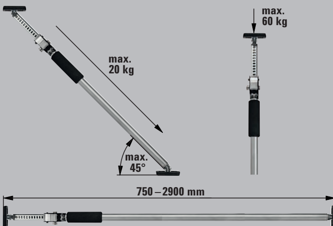
Telescopic drywall support ST
